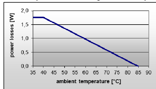
Permitted power losses during continuous operation
