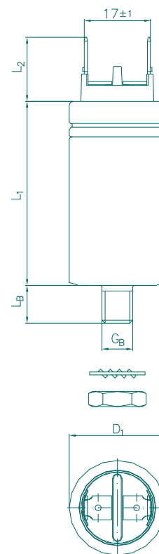
Outline drawing
