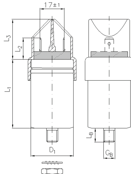
Outline drawing
