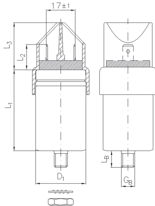
Outline drawing
