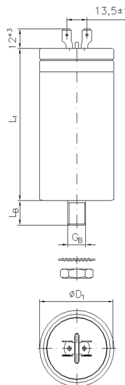
Outline drawing
