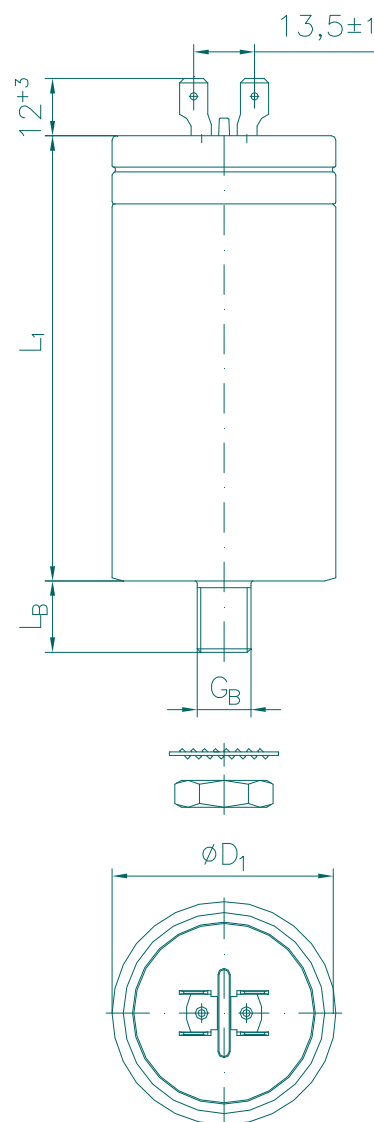
outline drawing
