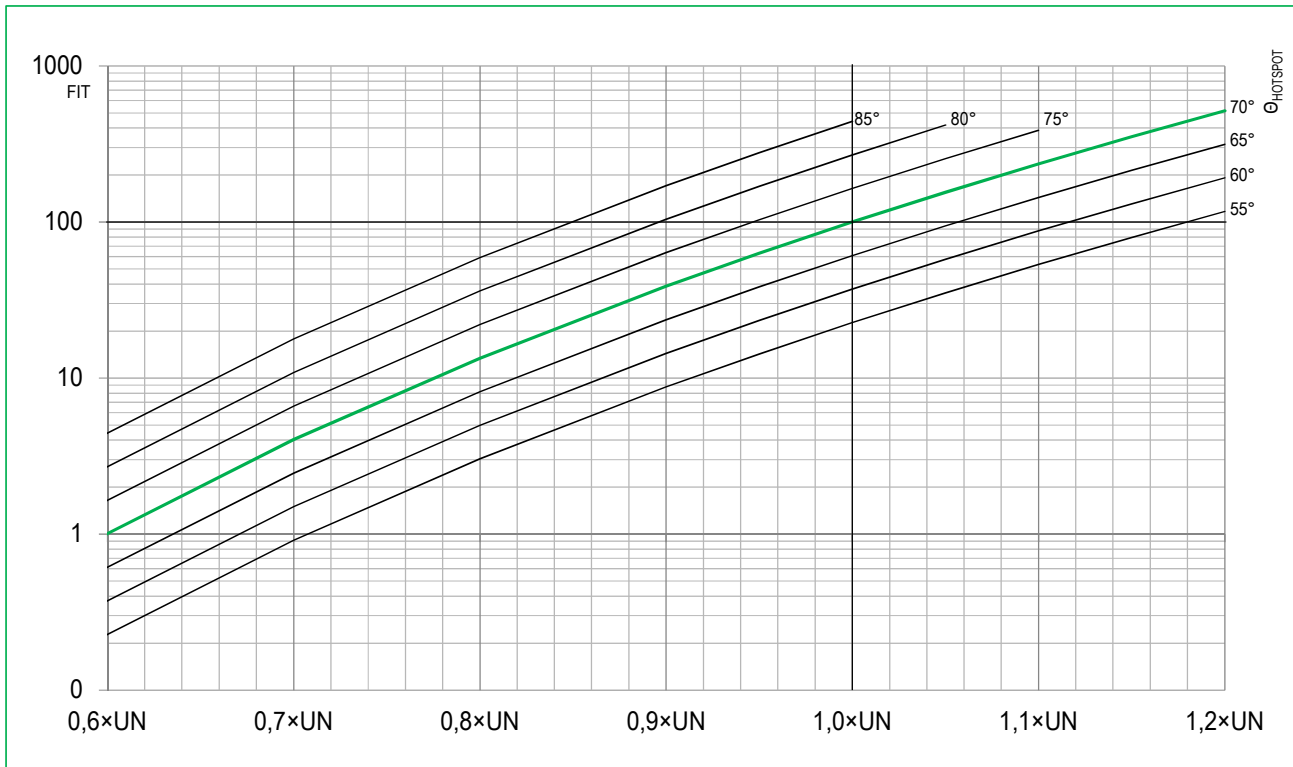
FIT-RATE versus HOTSPOT temperature and voltage
