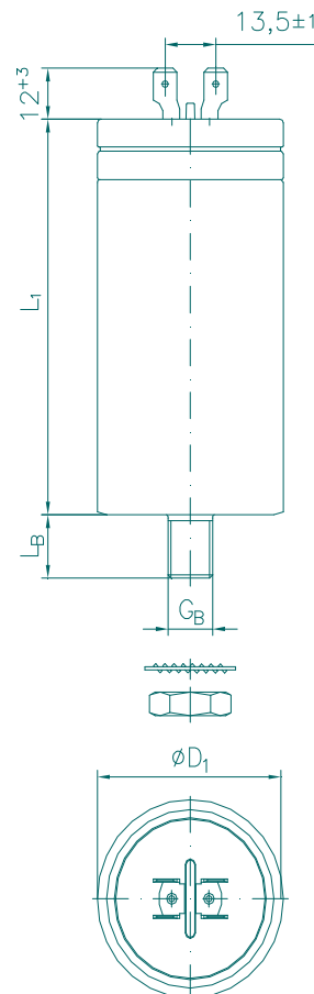
outline drawing
