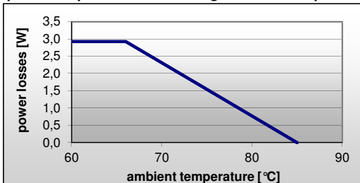
permitted power losses during continuous operation
