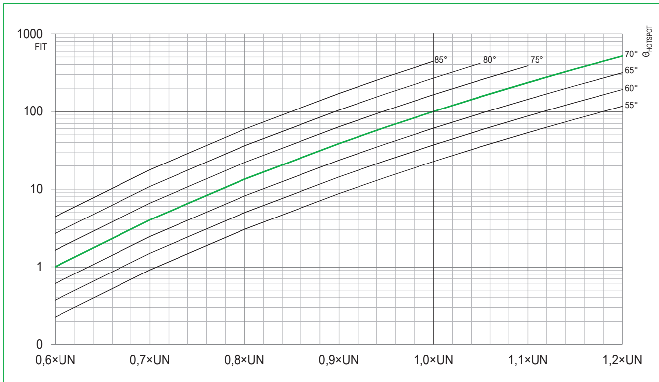
FIT-RATE versus HOTSPOT temperature and voltage
