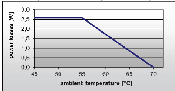
Permitted power losses during continuous operation
