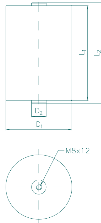
Outline drawing
