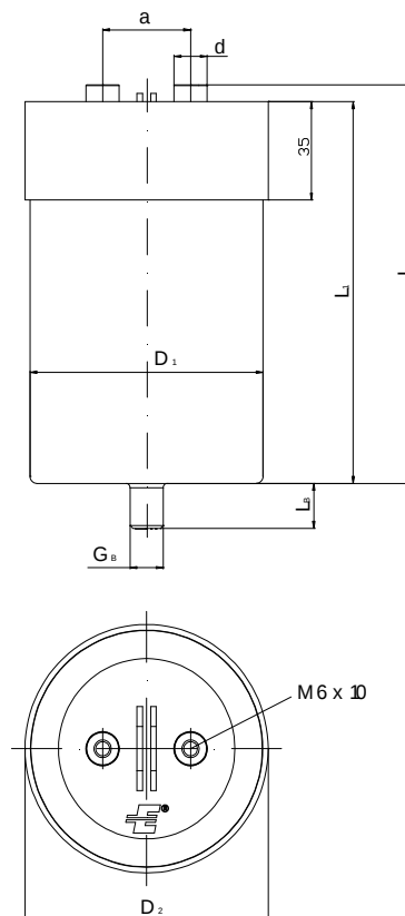
Outline drawing
