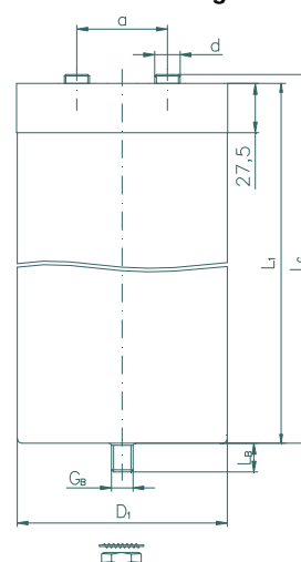
Outline drawing
