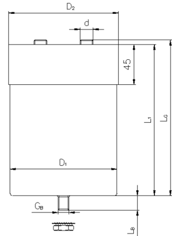
Outline drawing
