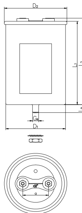
Outline drawing
