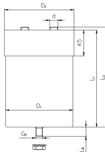
Outline drawing
