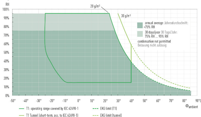
Humidity Classes T1 acc. to IEC 62498 1
