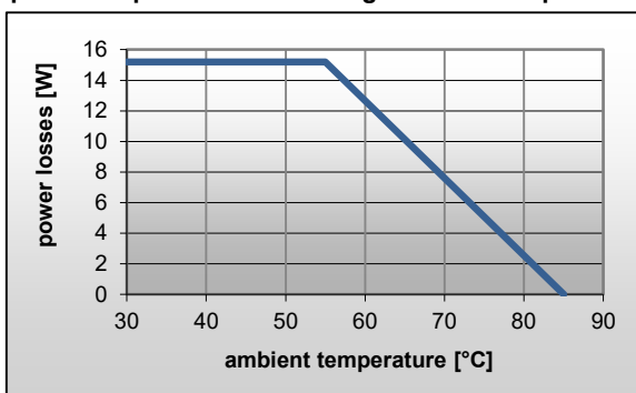
permitted power losses during continuous operation
