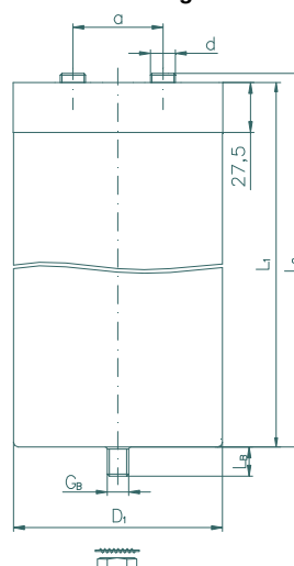
Outline drawing
