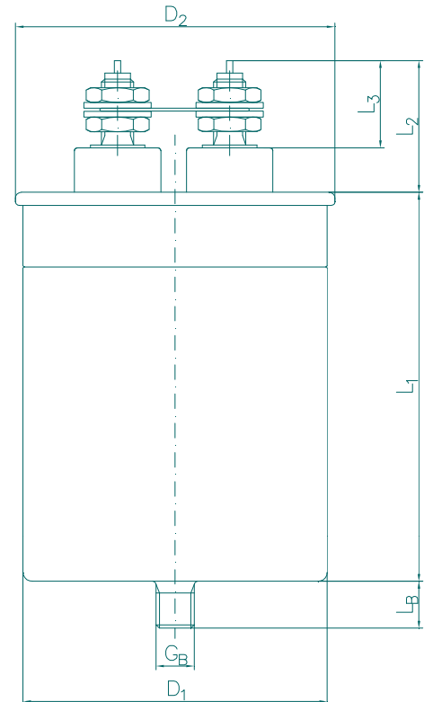
outline drawing
