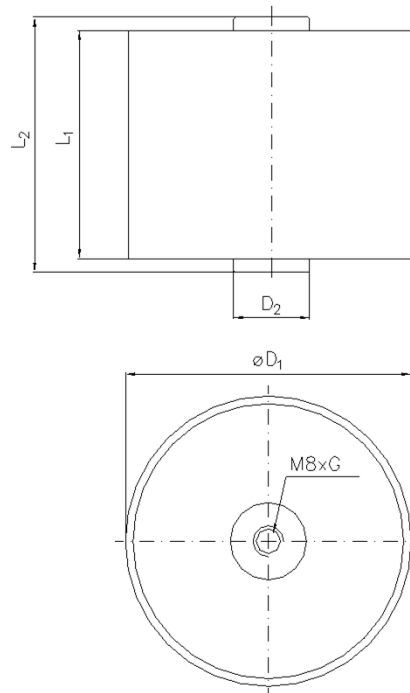
Outline drawing
