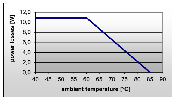
Permitted power losses during continuous operation
