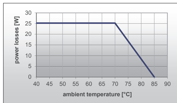
permitted power losses during continuous operation 1)
