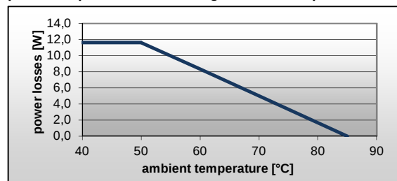
permitted power losses during continuous operation 1)
