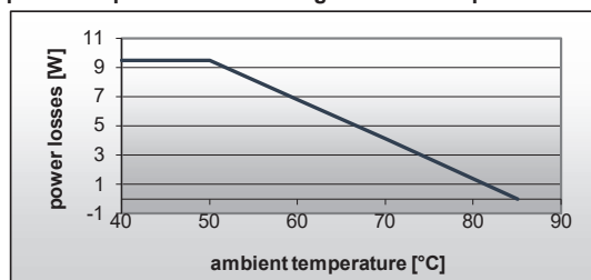
permitted power losses during continuous operation 2)
